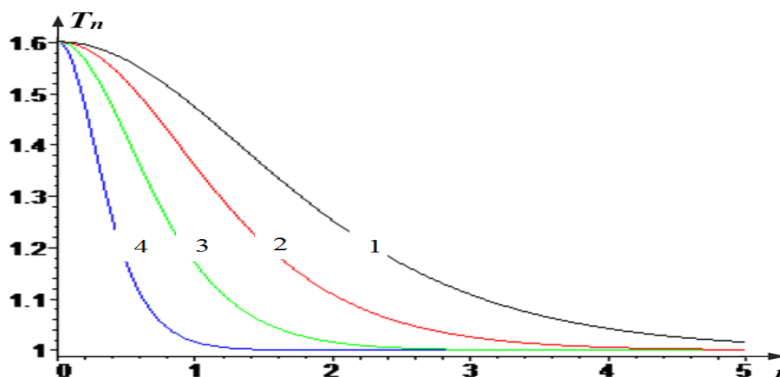
Fig. 3. Tension change T_c = T(t, \alpha_0) (related to T_n ) in t(\text{сек}) if f = 0.3 , \alpha_0 = 90^\circ different parameter values \gamma = \sqrt{ab} : 1 - \gamma = 0.5 , 2 - \gamma = 0.75 , 3 - \gamma = 1.25 , 4 - \gamma = 2.5
