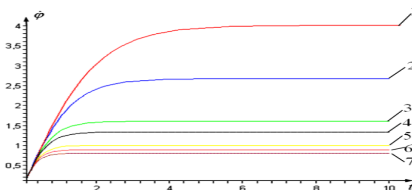
Figure 2. Time-dependent change in ball velocity – t(\text{sec}) at various parameter values \gamma = \sqrt{ab} : 1 - \gamma = 0.5 , 2 - \gamma = 0.75 , 3 - \gamma = 1.25 , 4 - \gamma = 1.5 , 5 - \gamma = 2.0 , 6 - \gamma = 2.25 , 7 - \gamma = 2.5
