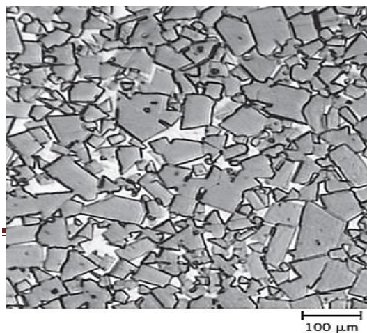
Figure 4. Photomicrograph of a WC-Co cemented carbide. Light areas are the cobalt matrix; dark regions, the particles of tungsten carbide. 100x.
