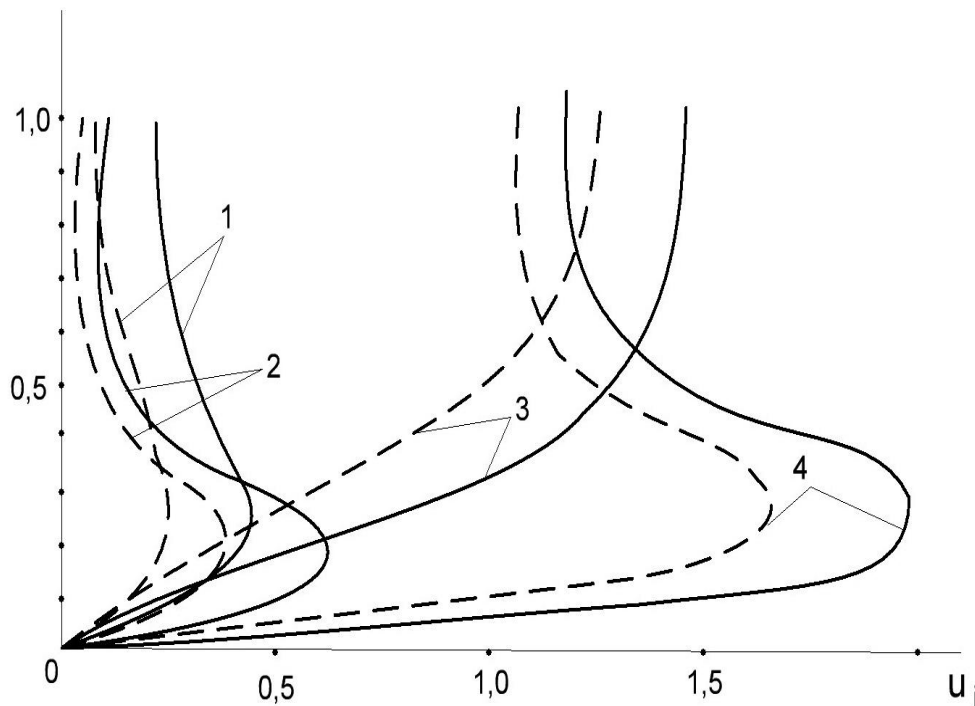
Fig. 1. Manifestation of Richardson effect for a two-phase mixture
