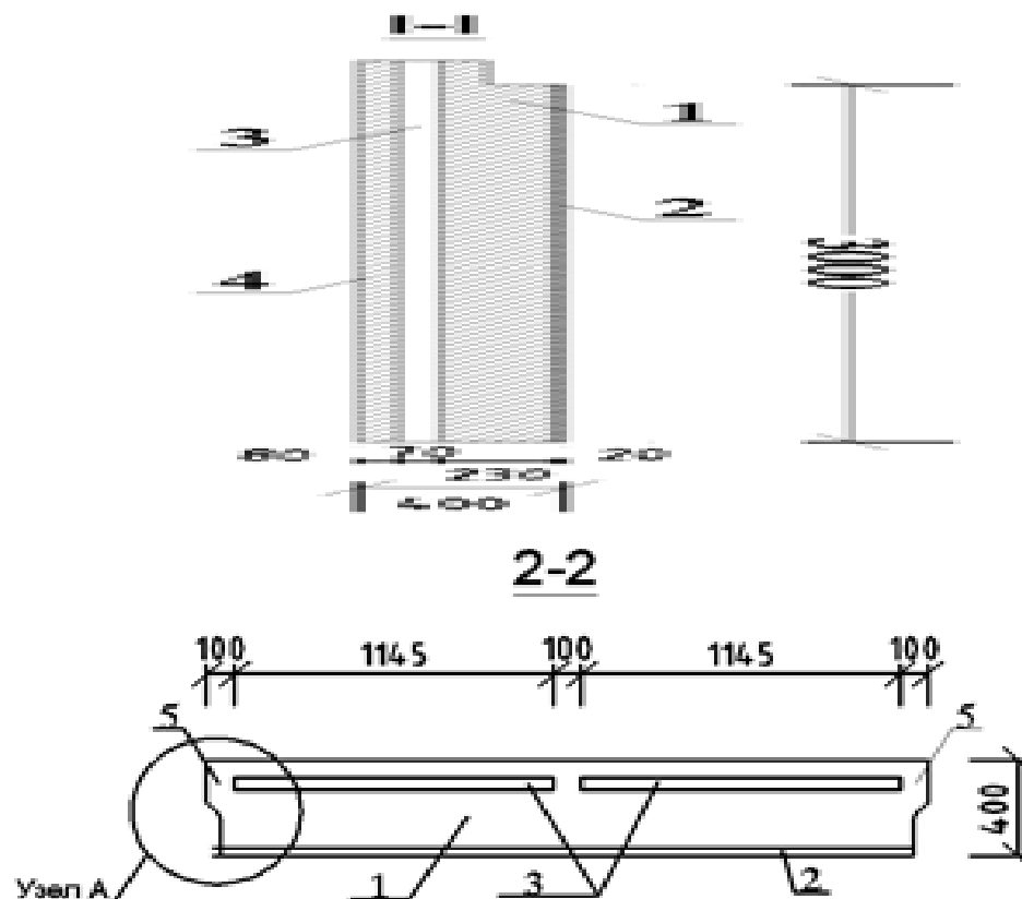
Figure: 1 Design of the experimental panel: 1-main part of the wall; 2-inner finishing layer; 3-air gap; 4-screen; 5-connecting ribs.
