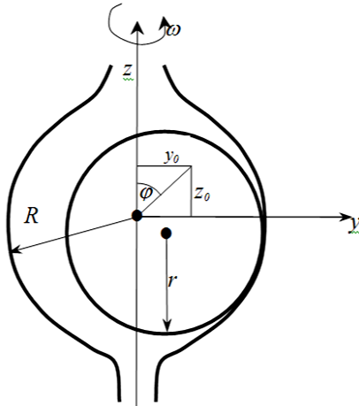
Figure 4. Schematic of an axisymmetric receptacle with a ball inside
