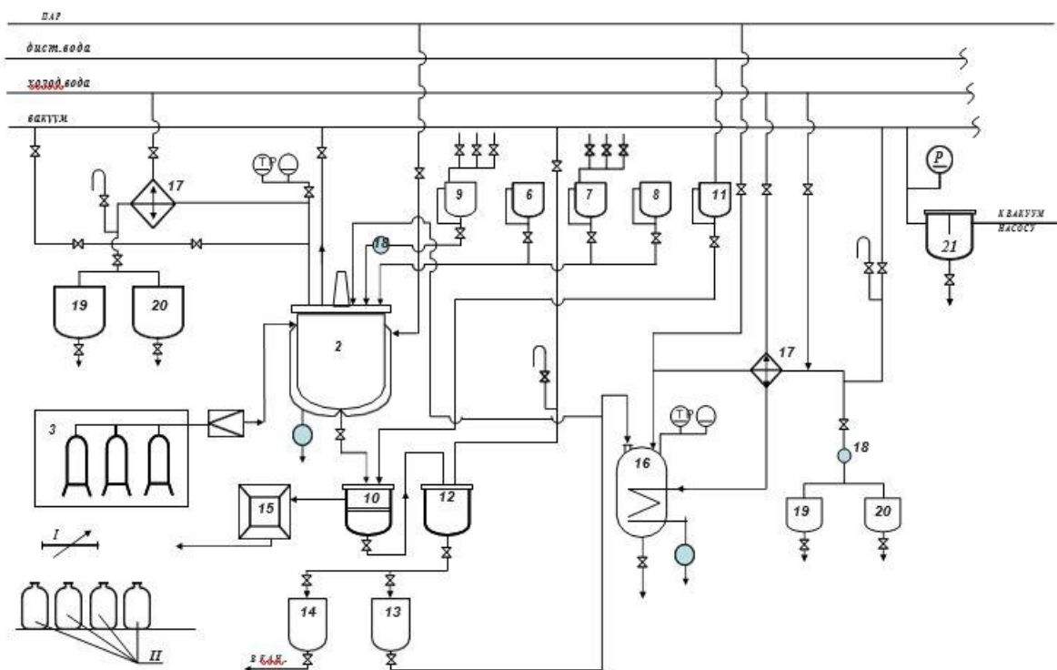
Figure 1. Technological scheme for the production of hexamethylenehexamethylenebis - [(p-ferrocenylphenyl)hydroxymethylene] -4- (pyrazolilo) -urea]
