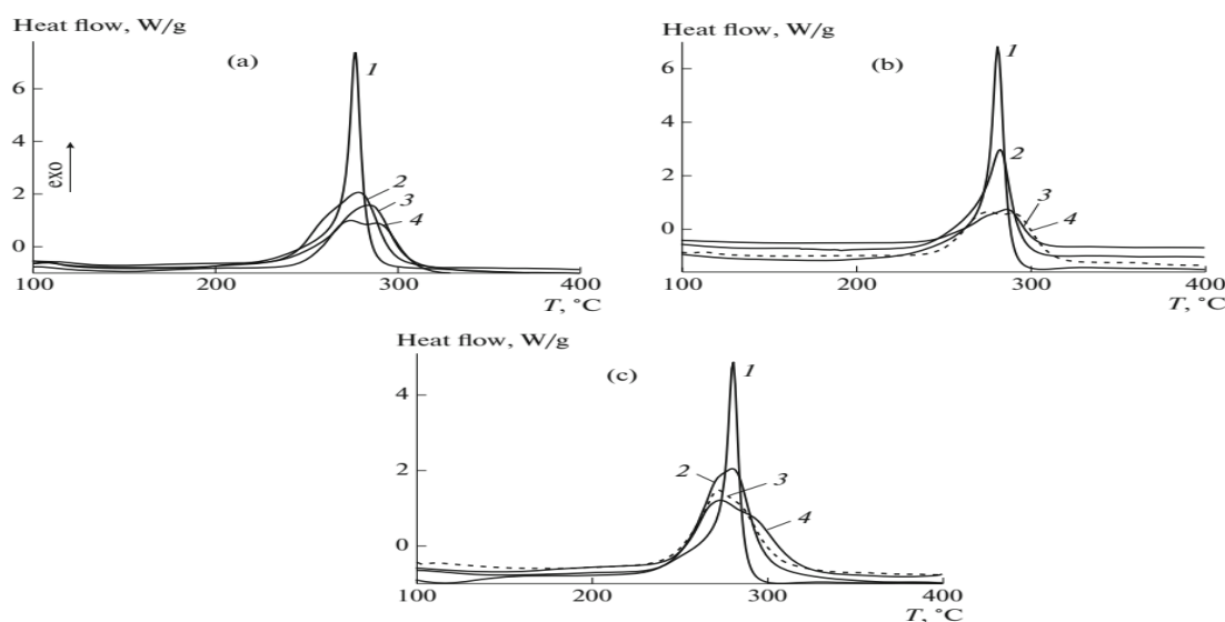
Fig. 1. Thermograms measured at a heating rate of 10^\circ\text{C}/\text{min} under inert atmosphere for the AN-AA copolymers synthesized in the presence of CTC-1 and AIBN at 80^\circ\text{C} . Molar ratio of AN : AA = (1) 98 : 2, (2) 95 : 5, (3) 93 : 7, and (4) 90 : 10; [\text{CTC-1}]_0 = (a, b) 5 \times 10^{-3} and (c) 1 \times 10^{-3} mol/L; [\text{AIBN}]_0 = (a, b) 1 \times 10^{-3} and (c) 5 \times 10^{-4} mol/L; the time of polymerization is (a) 24 and (b, c) 48 h.
