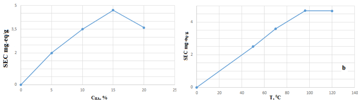
Figure 1. Dependence of the SEC of the anionite on the concentration of HA in the reaction mixture (a) and the process temperature (b)
