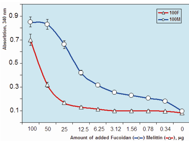
Figure 3. Change of turbidity of LMW fucoidan:melittin complex: 100 \mu l of 0.1% fucoidan solution mixed with equal volume of indicated amount melittin solution (line “100 F”) and 100 \mu l of 0.1% melittin solution mixed with equal volume of indicated amount fucoidan solution (line “100 M”).
