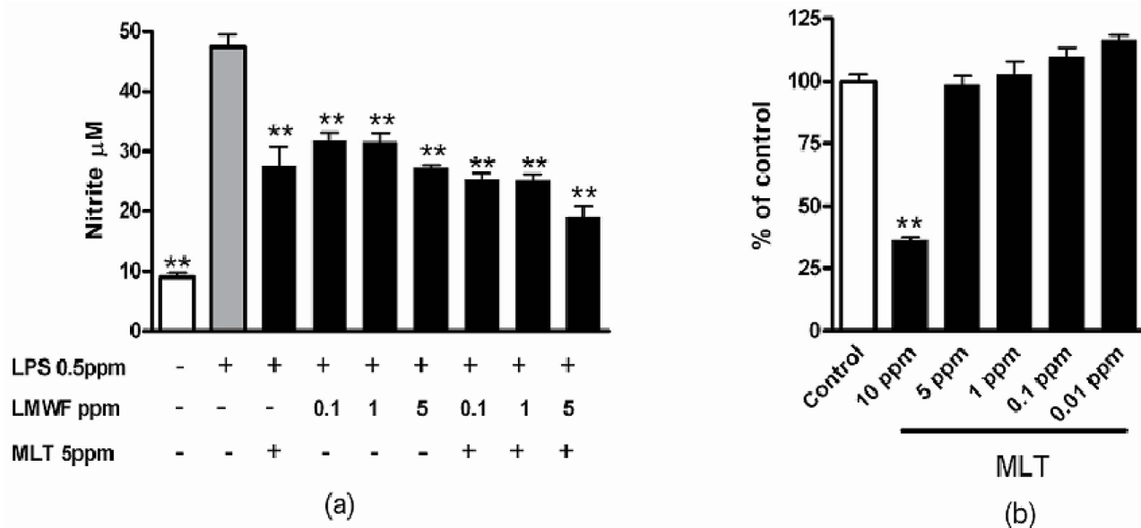
Figure 5. Inhibition of lipopolysaccharide (LPS)-induced production of nitric oxide (a) by LMW fucoidan and melittin and cytotoxicity of melittin on macrophage of Raw 264.7 (b). As indicated, macrophage cell line RAW 264.7 was treated with LPS, LMW fucoidan and melittin. After 24 hours incubation, the amounts of NO in the media were measured as nitrite by Griess reagent. * P < 0.05 ; ** P < 0.01 .
