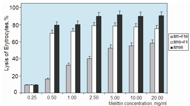
Figure 4. Hemolytic activity of LMW fucoidan:melittin complexes (melittin:fucoidan relation 1:10 “M1 + F10” and 10:1 “M10 + F1”) and free melittin (“M100”). Concentration of complexes indicated as melittin content. Hemolytic activity was calculated relative to lytic activity of Triton X-100 (0.05%).
