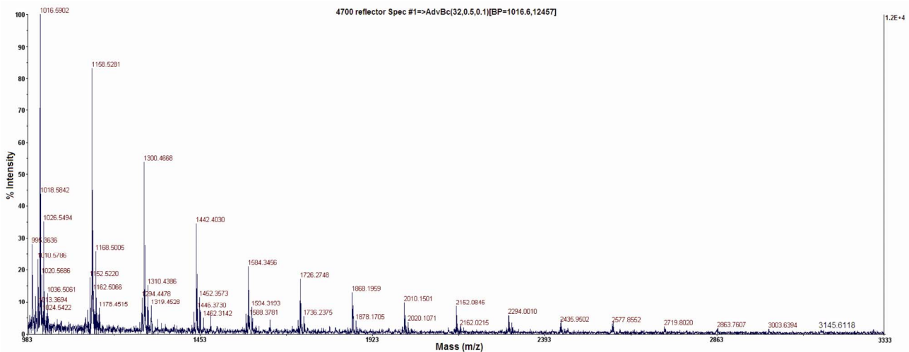
Figure 2. MALDI-TOF/TOF spectrum of LMW fucoidan obtained by free radical depolymerization.
