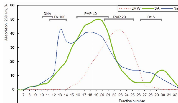
Figure 1. A molecular heterogeneity of fucoidan and its low molecular forms on Toyopearl HW-55 column. "Nat"—native fucoidan, "SA"—low molecular form obtained by sulfuric acid hydrolysis, "LMW"—low molecular form obtained by free radical depolymerization method. Elution volume of used molecular size markers are indicated as: DNA—genomic DNA ( >10^3 kDa); Dx 100 and Dx 6—dextranes 100 and 6 kDa; PVP 40 and PVP 20 - 40 and 20 kDa polyvinyl pyrrolidones.
